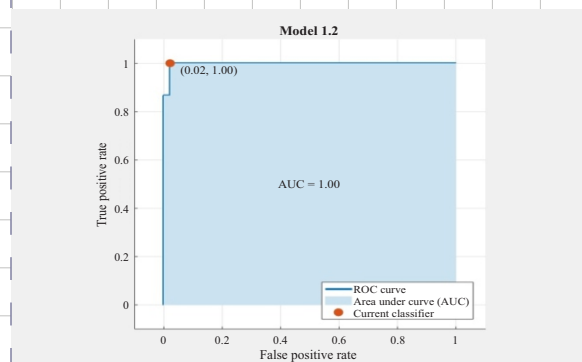
Fig. 12. ROC curve of Healthy leaves as Positive Class
