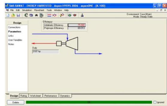
Figure 5: SMS Rawat Power Generation ASPEN HYSYS
