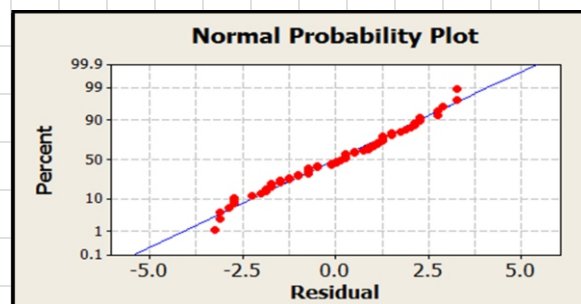
Fig. 4. Normal probability plot for residuals
