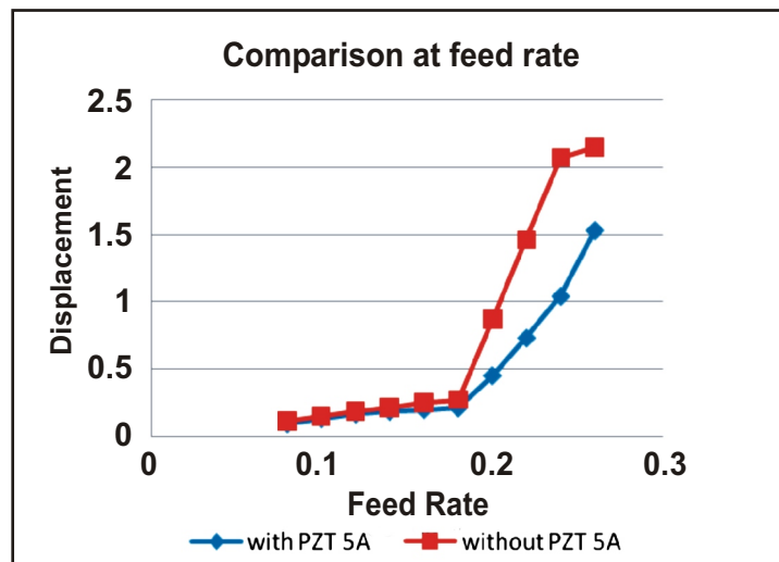
Figure 7 : Comparison between with and without pzt cutting tool at feed rate
