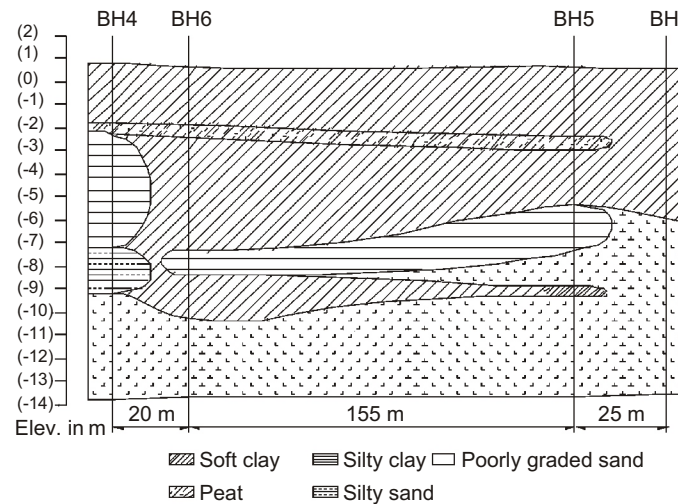
Figure 3 : Soil profile of case 5
