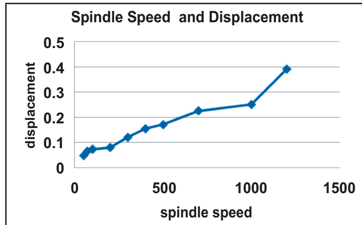
Figure 3 : Displacement and spindle speed of simple cutting tool
